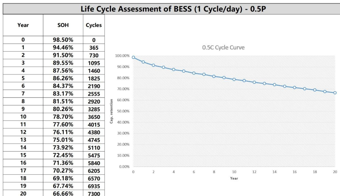
Fig.3 Degradation Curve in 0.5P, 1CPD Working Condition
