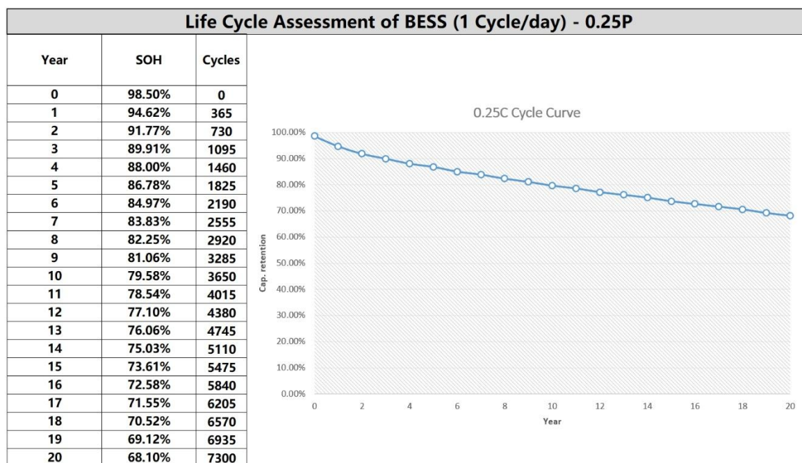
Fig.1 Degradation Curve in 0.25P, 1CPD Working Condition
