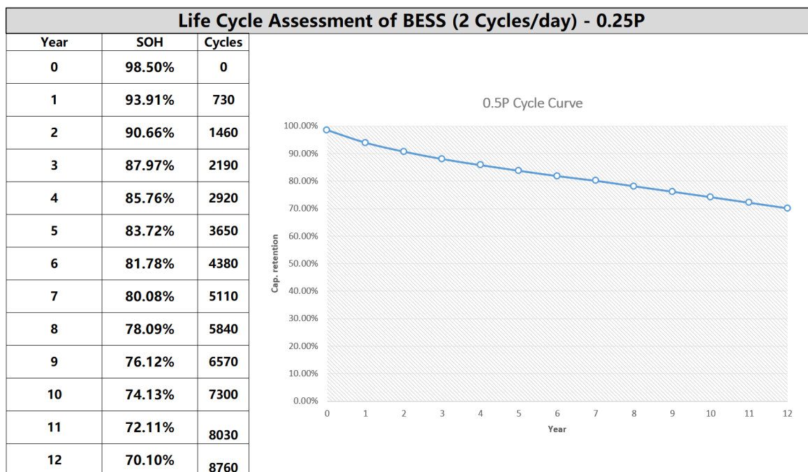
Fig.2 Degradation Curve in 0.25P, 2CPD Working Condition
