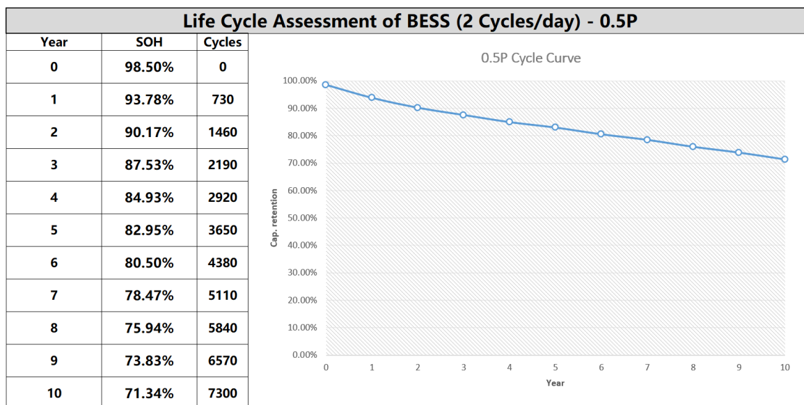
Fig.4 Degradation Curve in 0.5P, 2CPD Working Condition
